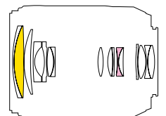
B018 Optical Construction ■ Hybrid Aspherical Element ■ LD Element
